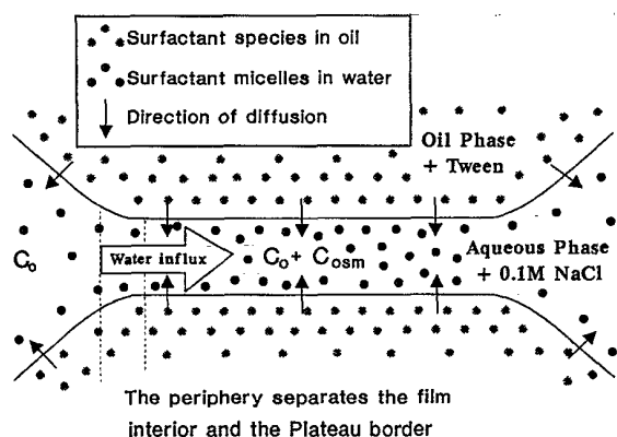
FIG. 4. Schematic presentation of the origin of the increased osmotic pressure between the film surfaces.
